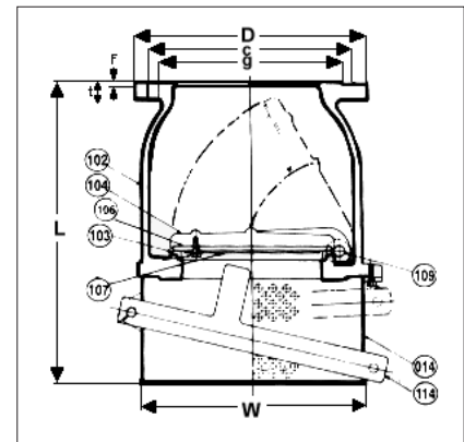
SIZE 200 - 400 mm
